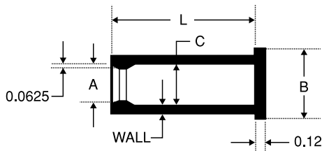
SFC SERIES SILICONE FLANGE CAPS
